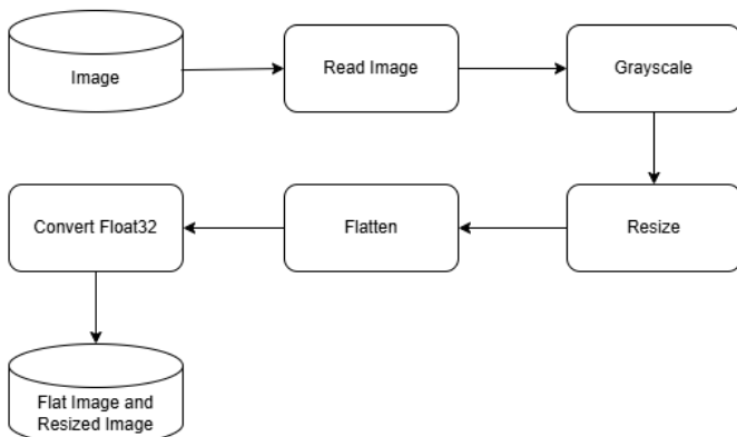
Gambar 3. Tahapan preprocessing gambar.
