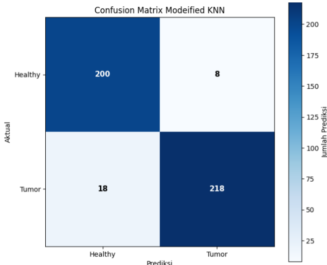
Gambar 9. Hasil Confusion Matrix Modified KNN
